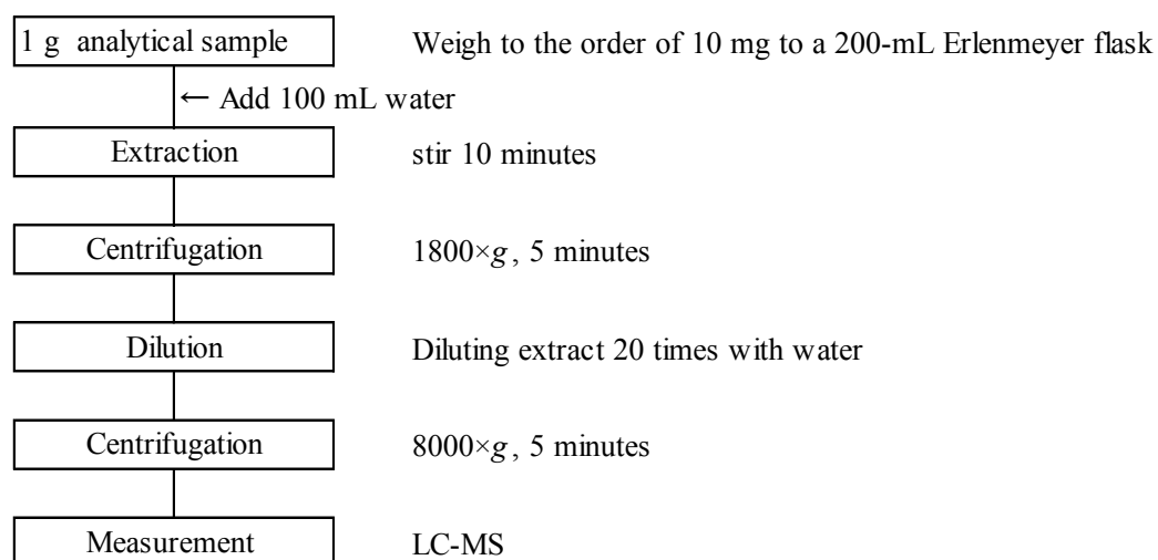
Scheme 1 Flow sheet for sulfamic acid in solid fertilizers
